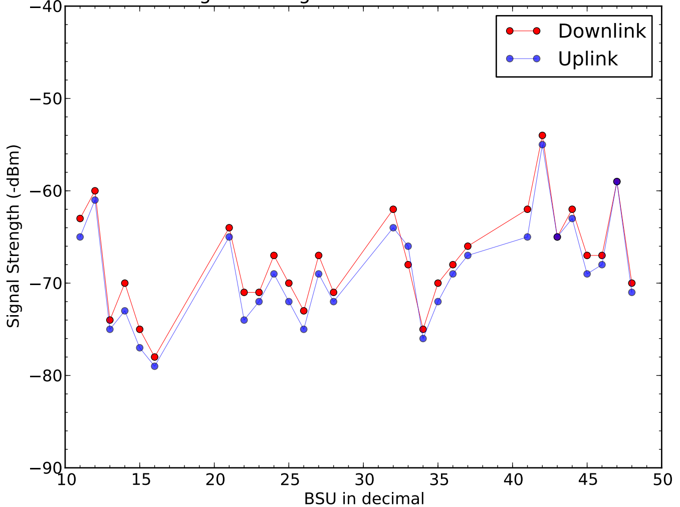
Signal Strength of BSU on 2016-08-02
