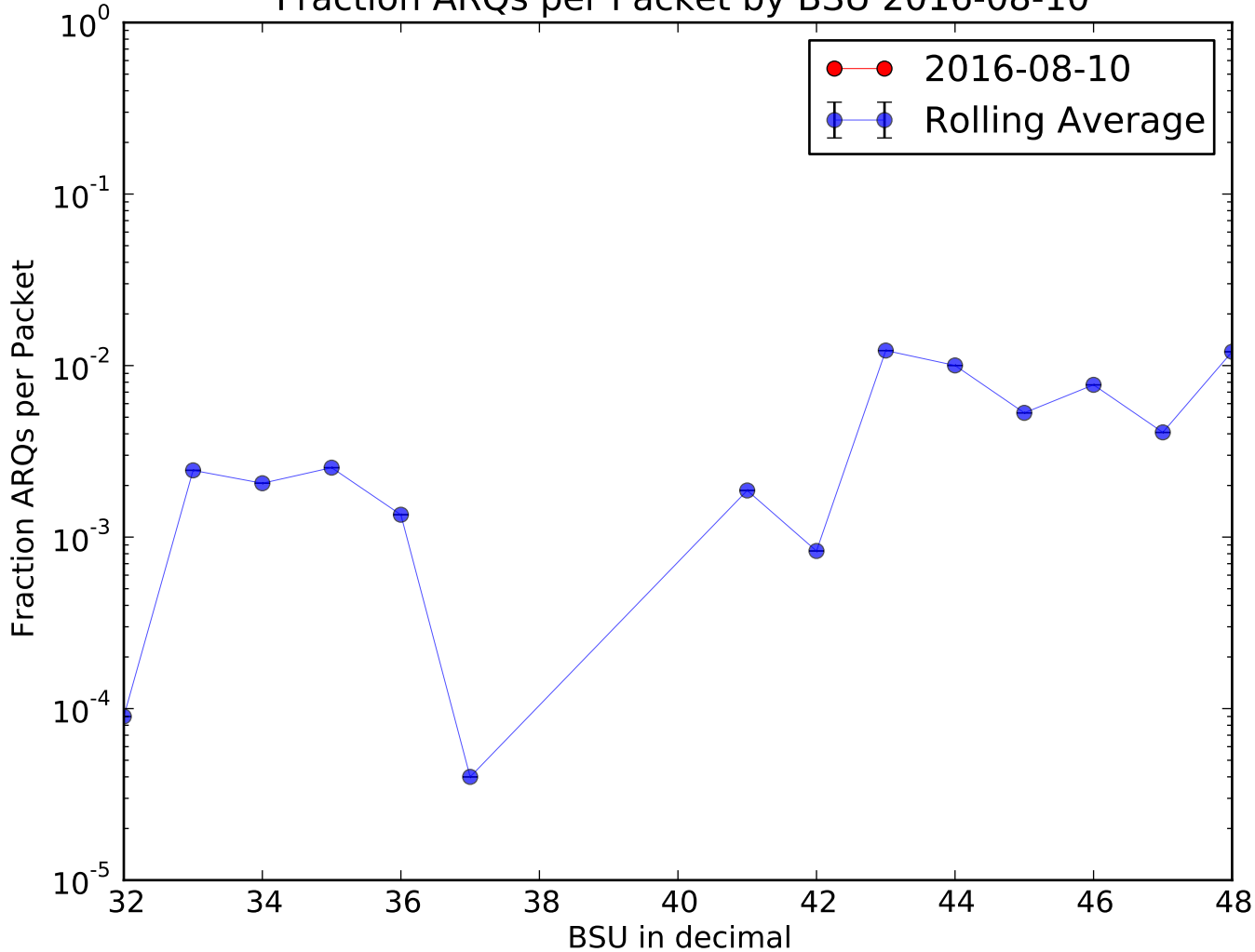
Fraction ARQs per Packet by BSU 2016-08-10
