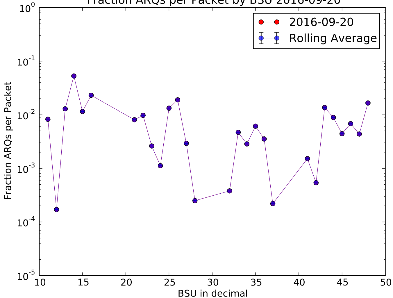
Fraction ARQs per Packet by BSU 2016-09-20
