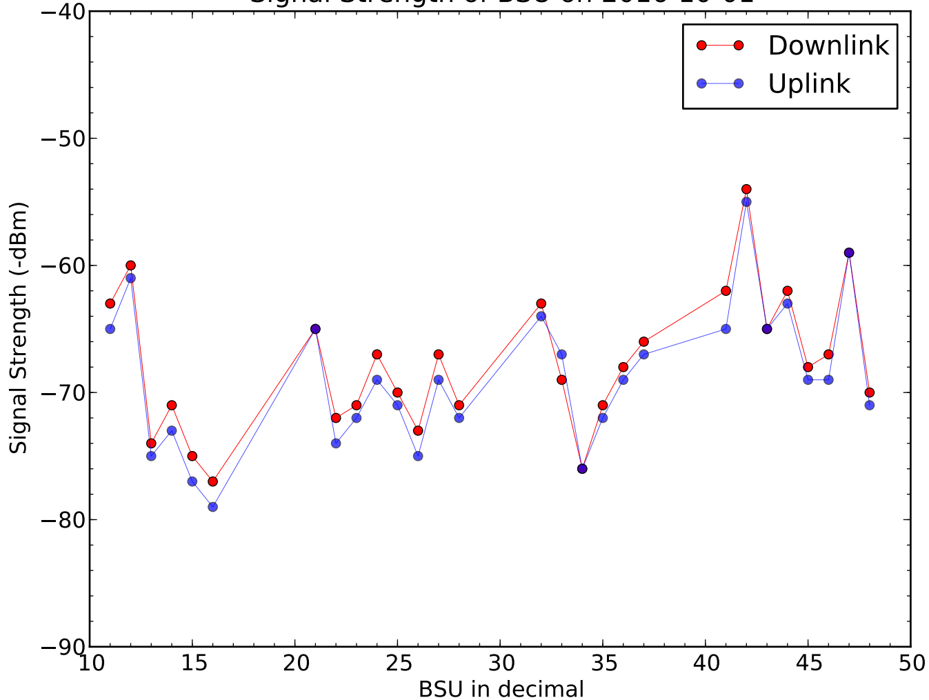
Signal Strength of BSU on 2016-10-01
