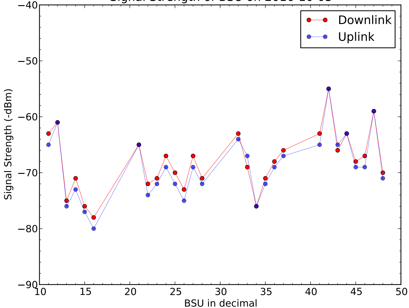
Signal Strength of BSU on 2016-10-03
