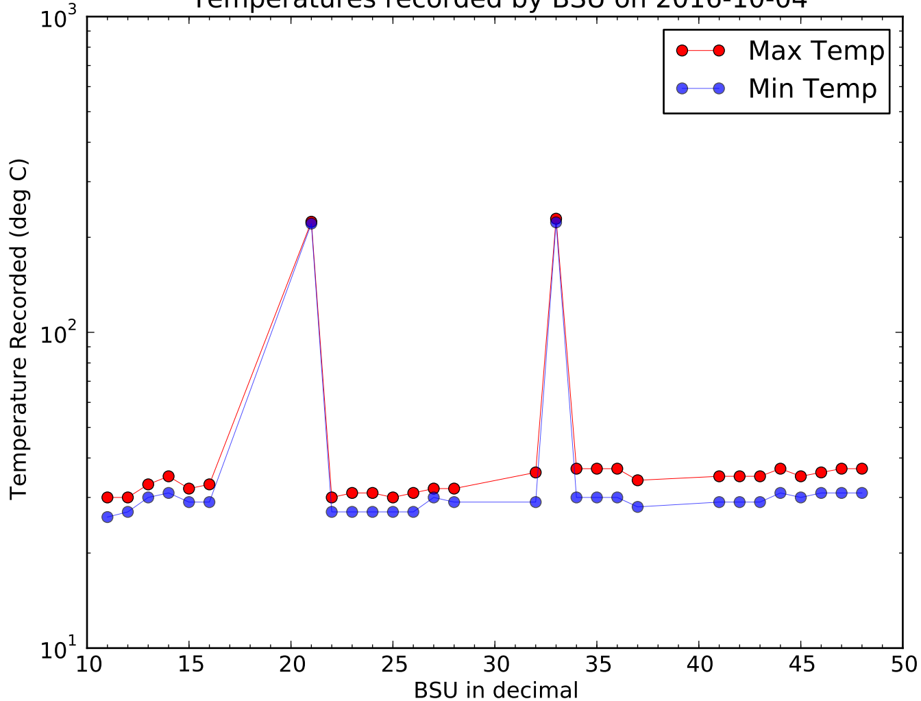
Temperatures recorded by BSU on 2016-10-04
