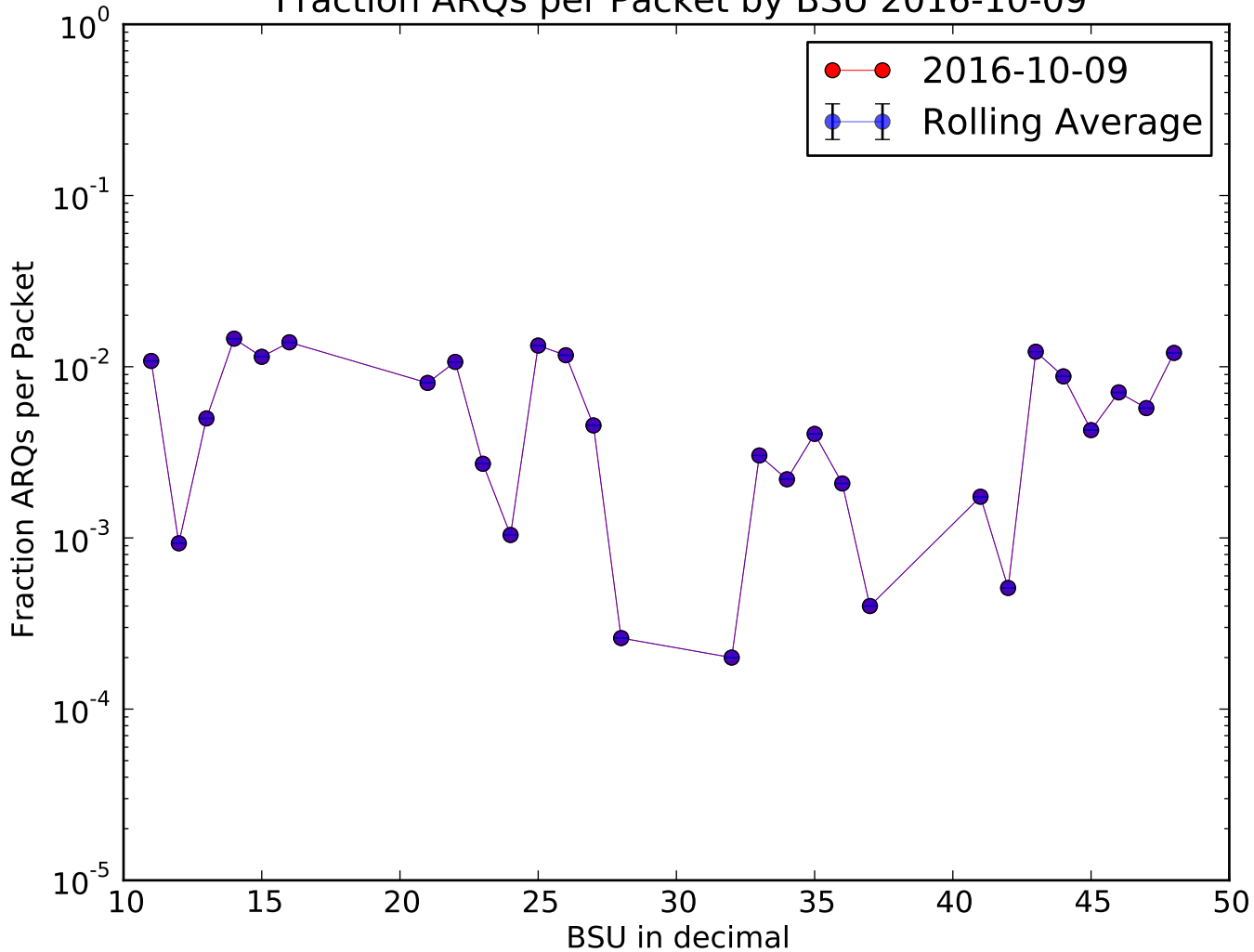
Fraction ARQs per Packet by BSU 2016-10-09
