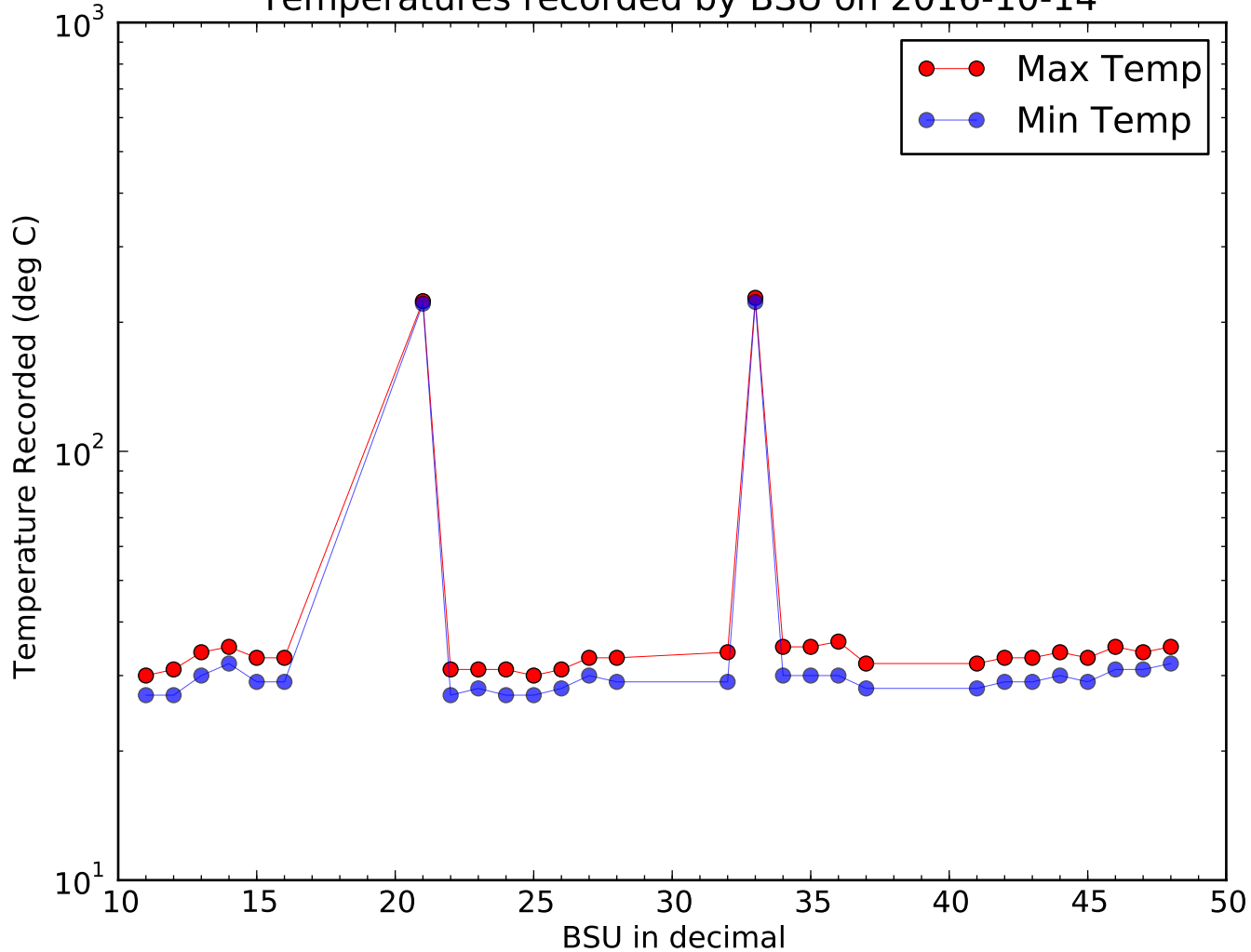
Temperatures recorded by BSU on 2016-10-14
