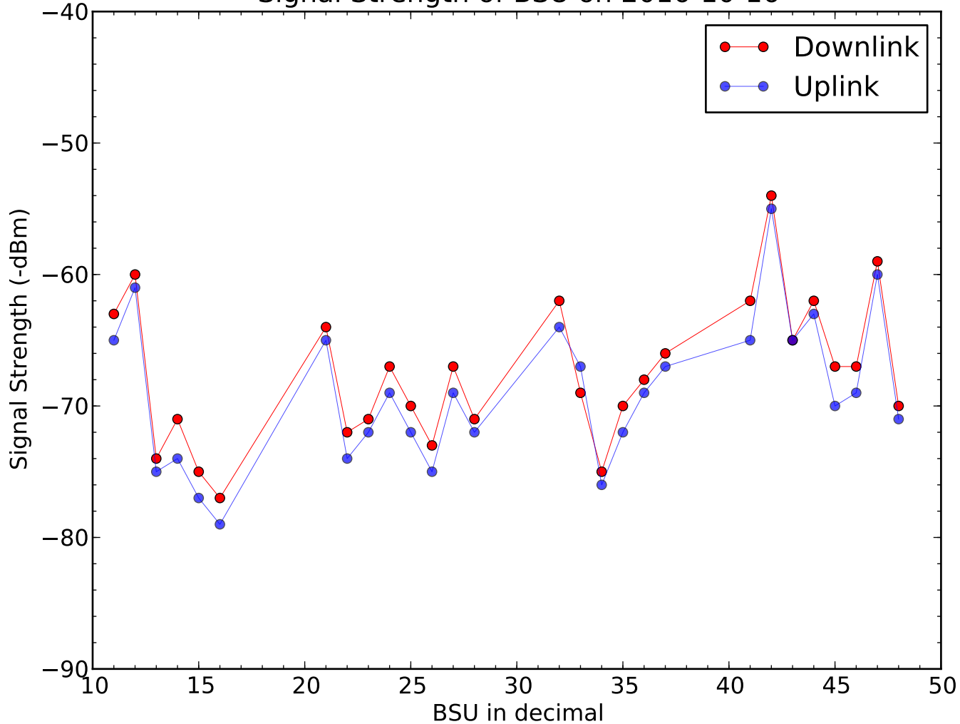
Signal Strength of BSU on 2016-10-16
