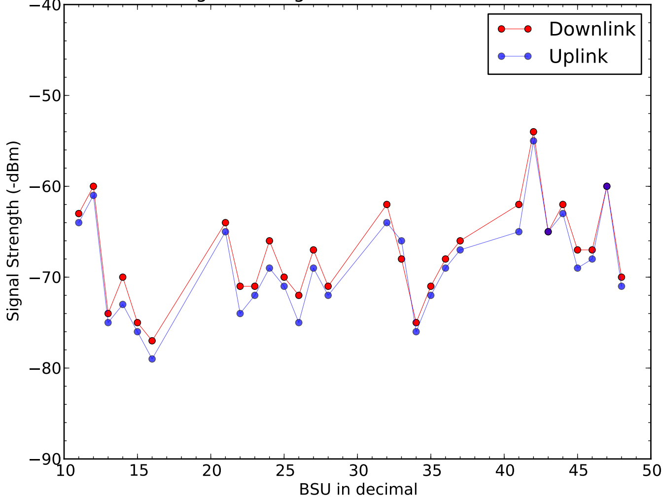
Signal Strength of BSU on 2016-10-18
