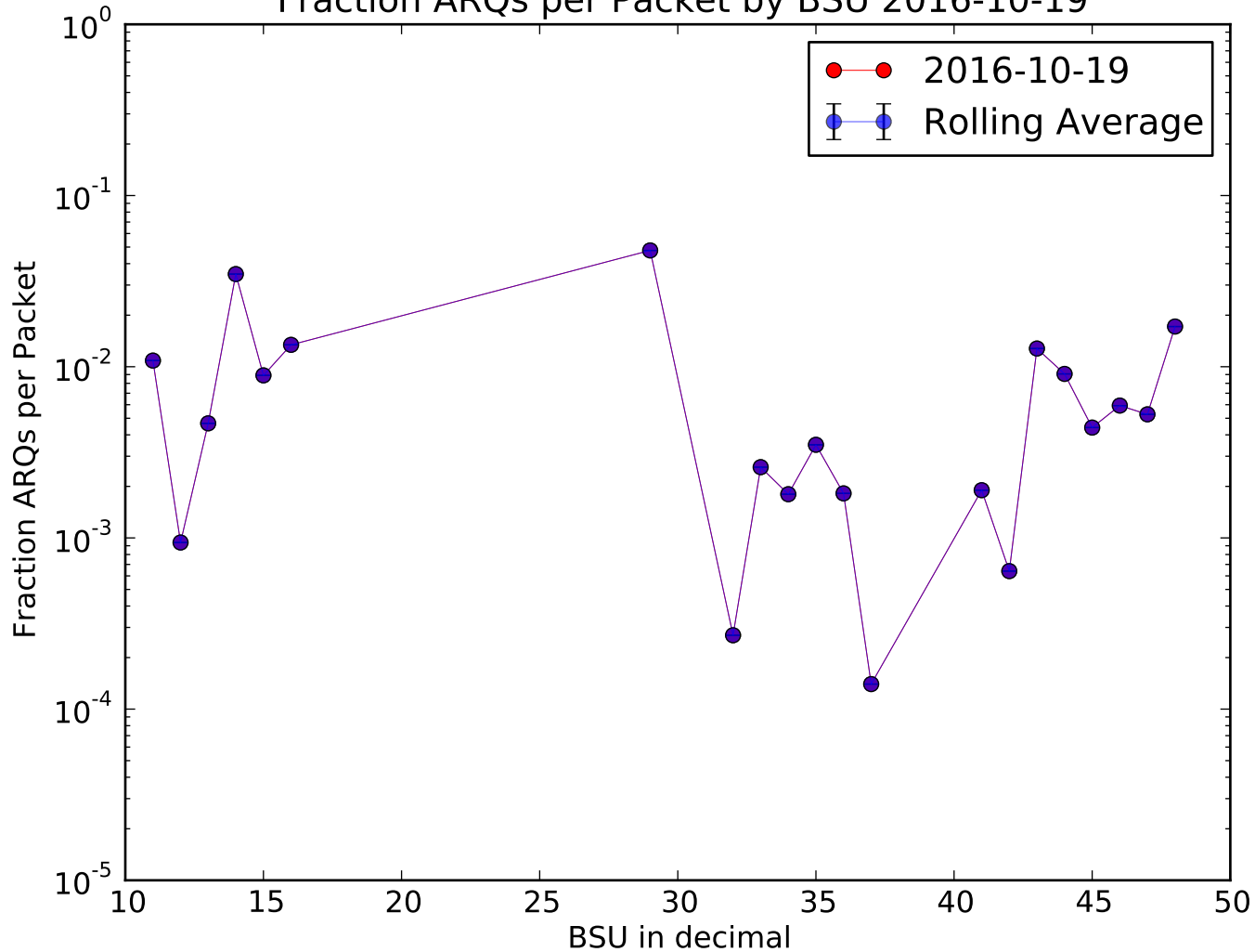
Fraction ARQs per Packet by BSU 2016-10-19
