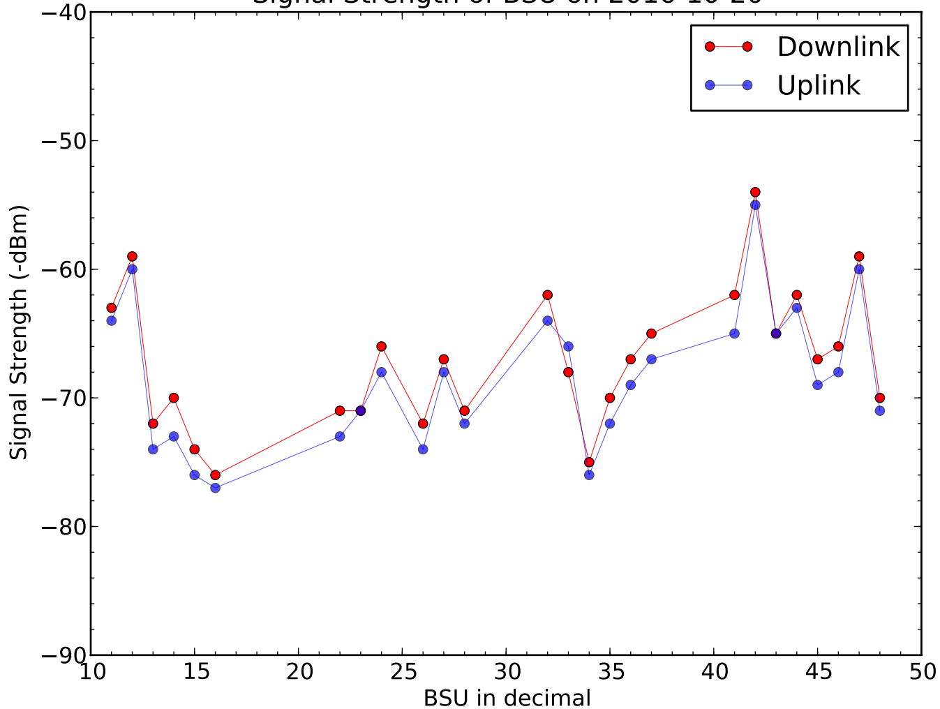
Signal Strength of BSU on 2016-10-20
