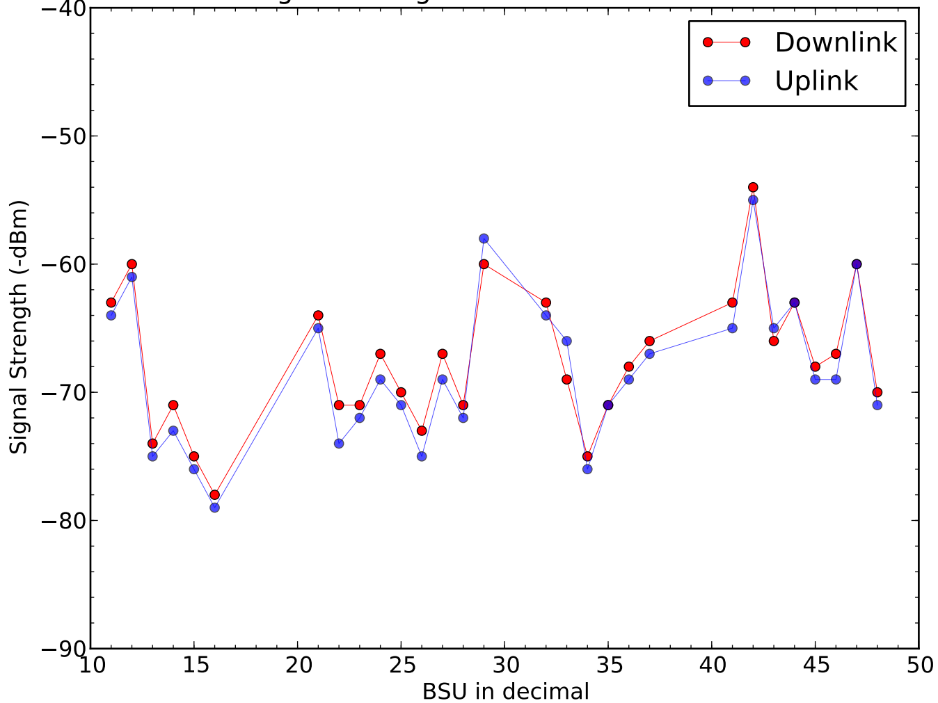
Signal Strength of BSU on 2016-10-22
