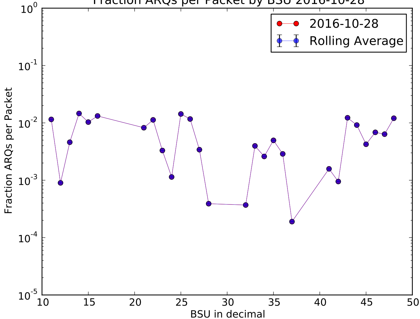
Fraction ARQs per Packet by BSU 2016-10-28
