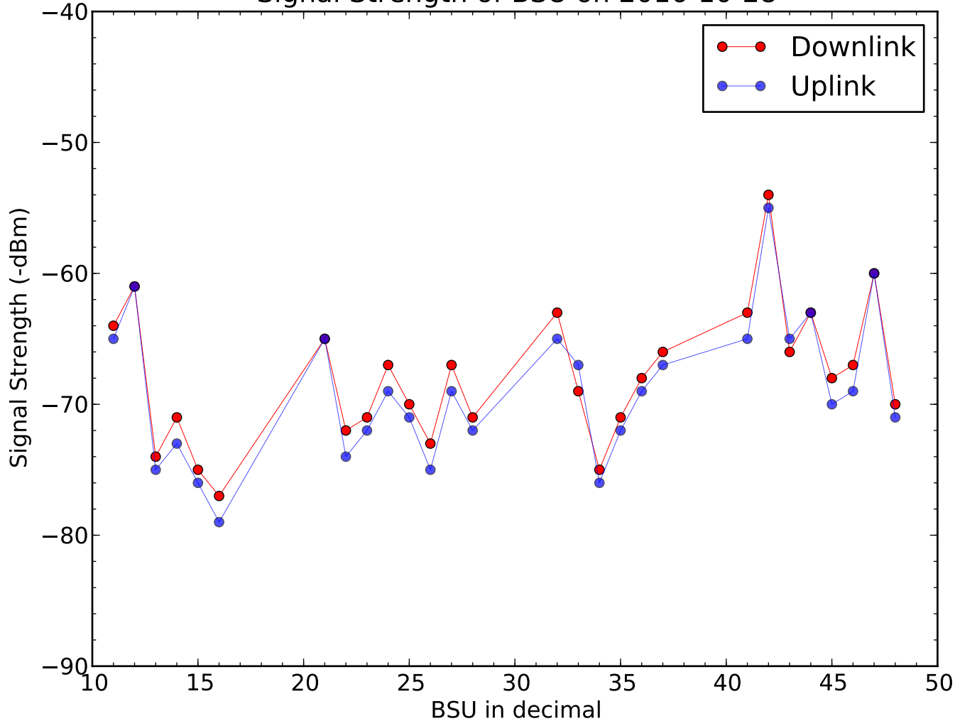
Signal Strength of BSU on 2016-10-28
