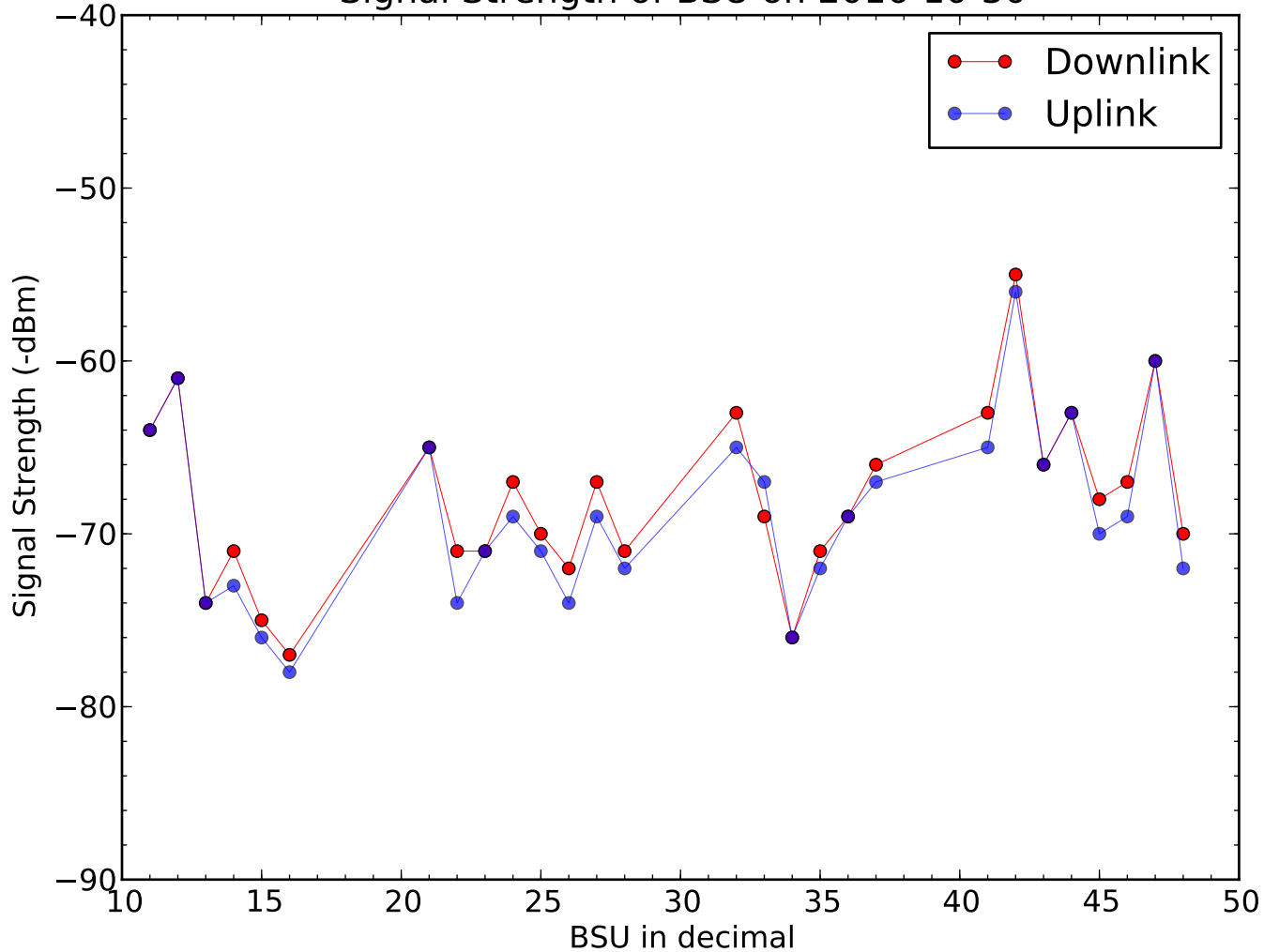
Signal Strength of BSU on 2016-10-30
