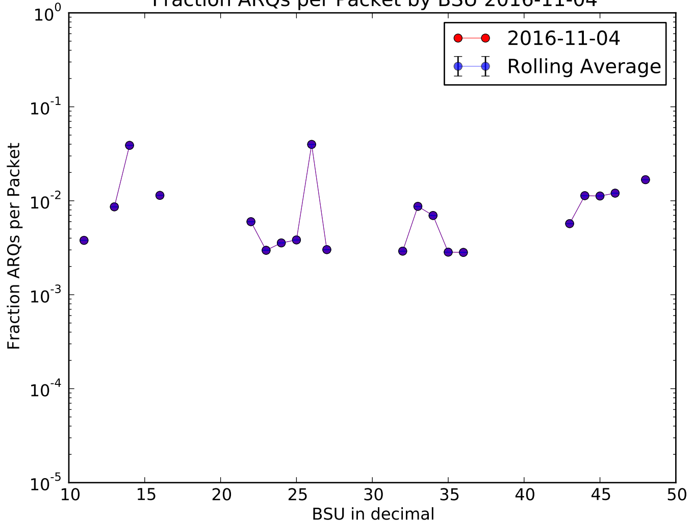
Fraction ARQs per Packet by BSU 2016-11-04
