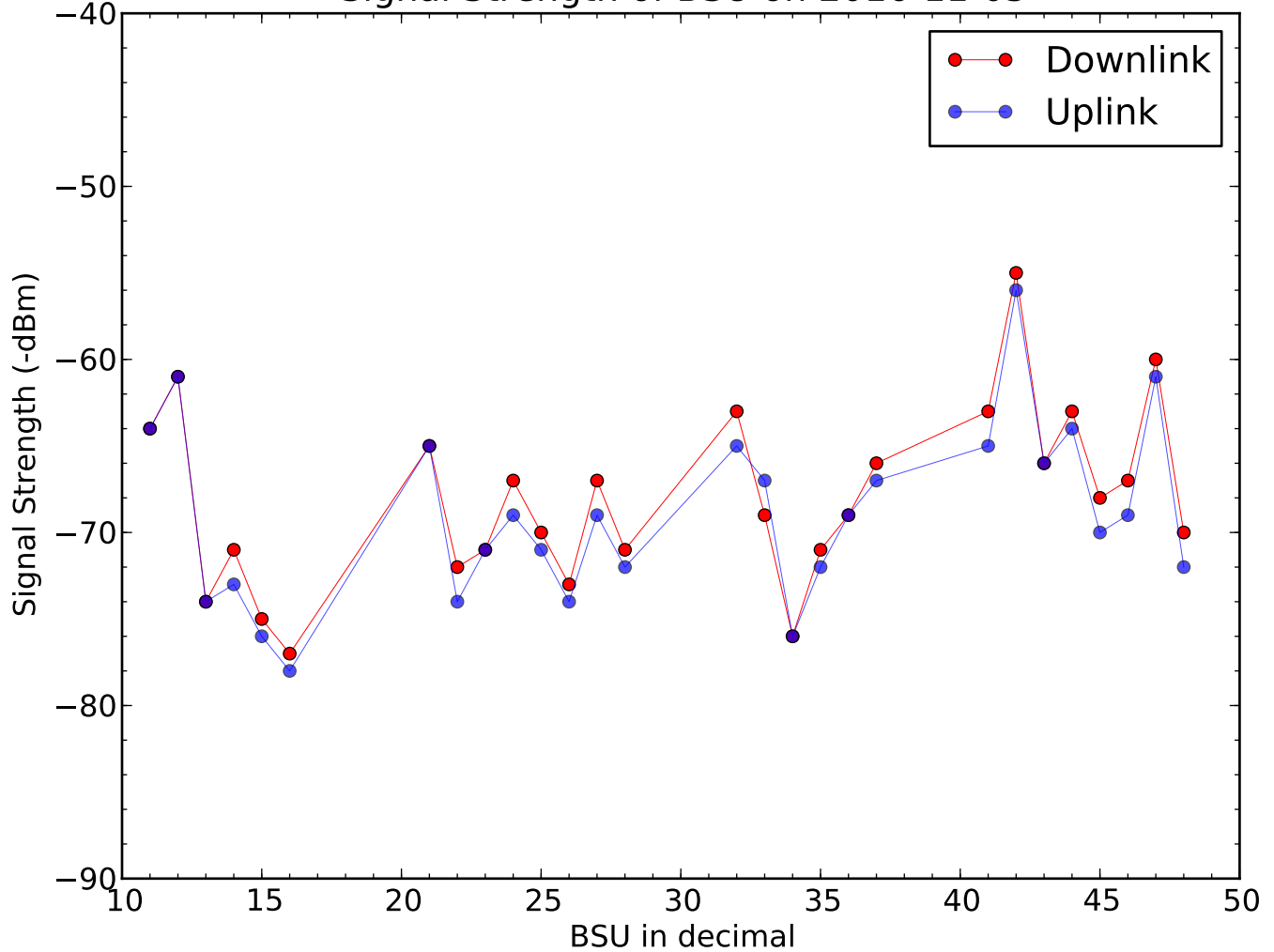
Signal Strength of BSU on 2016-11-05
