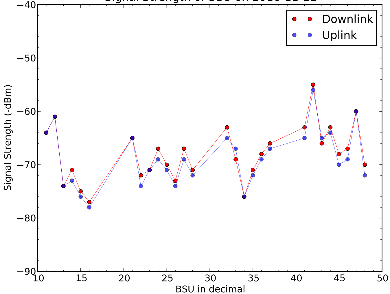
Signal Strength of BSU on 2016-11-11
