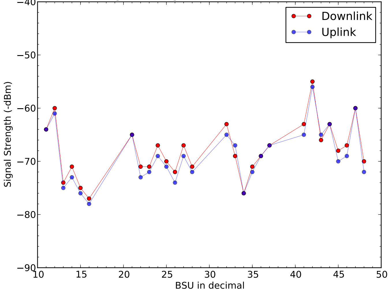
Signal Strength of BSU on 2016-11-14
