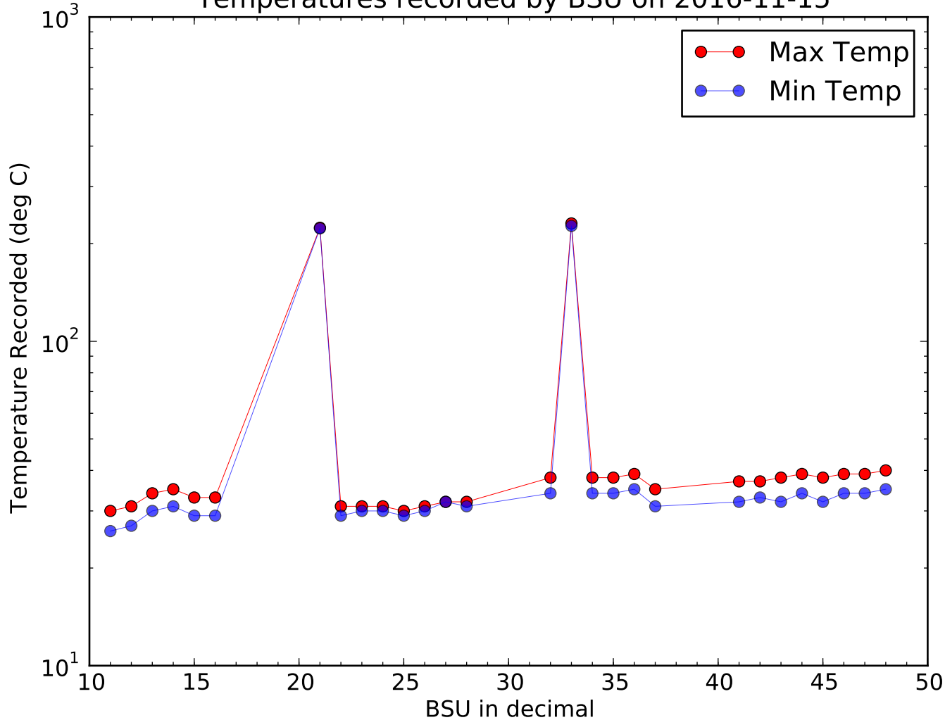
Temperatures recorded by BSU on 2016-11-15
