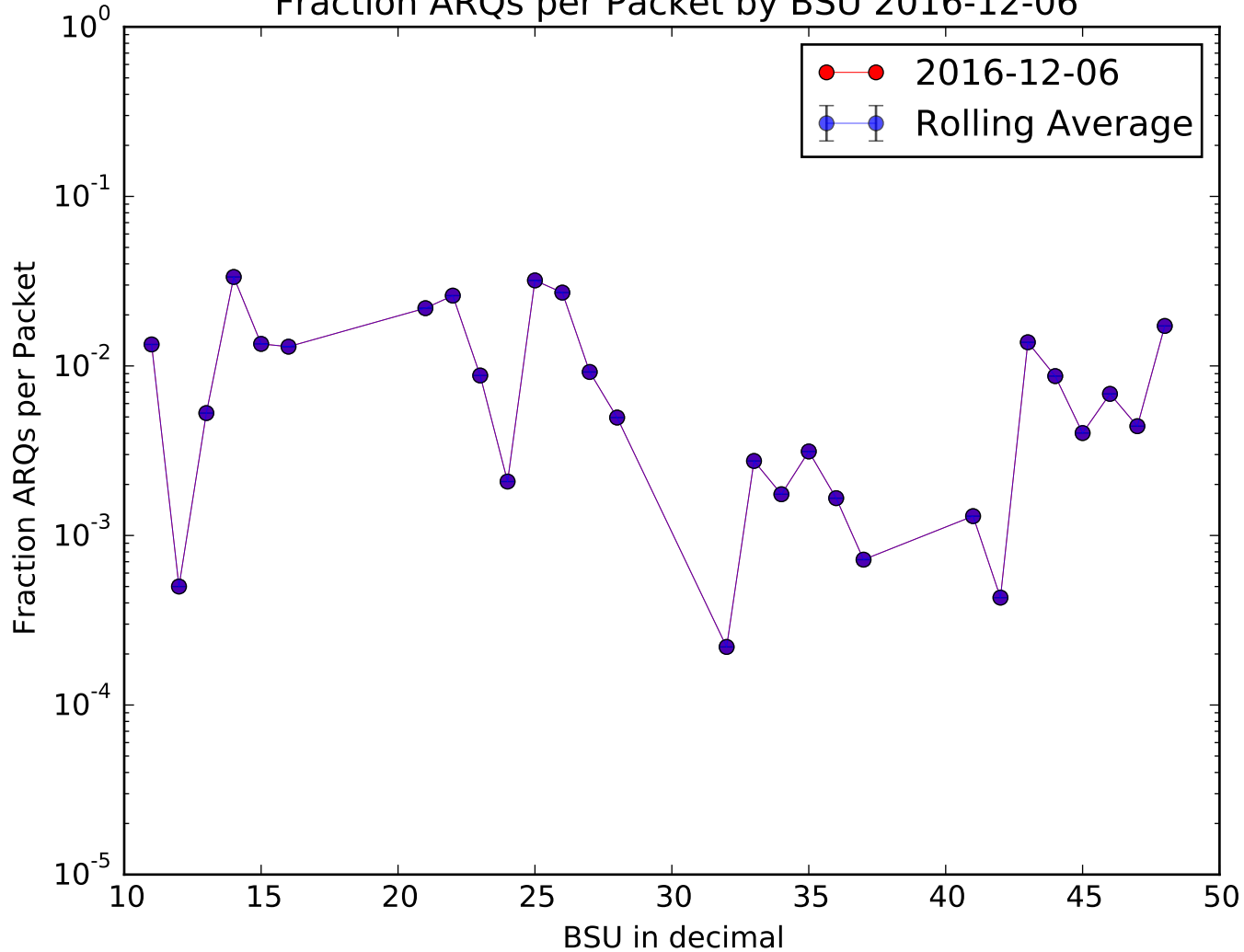
Fraction ARQs per Packet by BSU 2016-12-06
