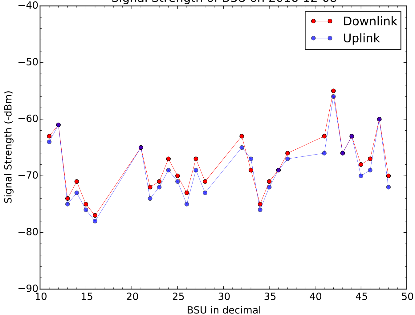
Signal Strength of BSU on 2016-12-08
