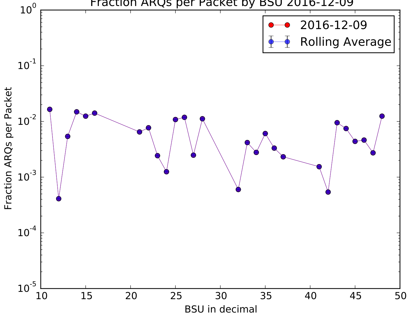
Fraction ARQs per Packet by BSU 2016-12-09
