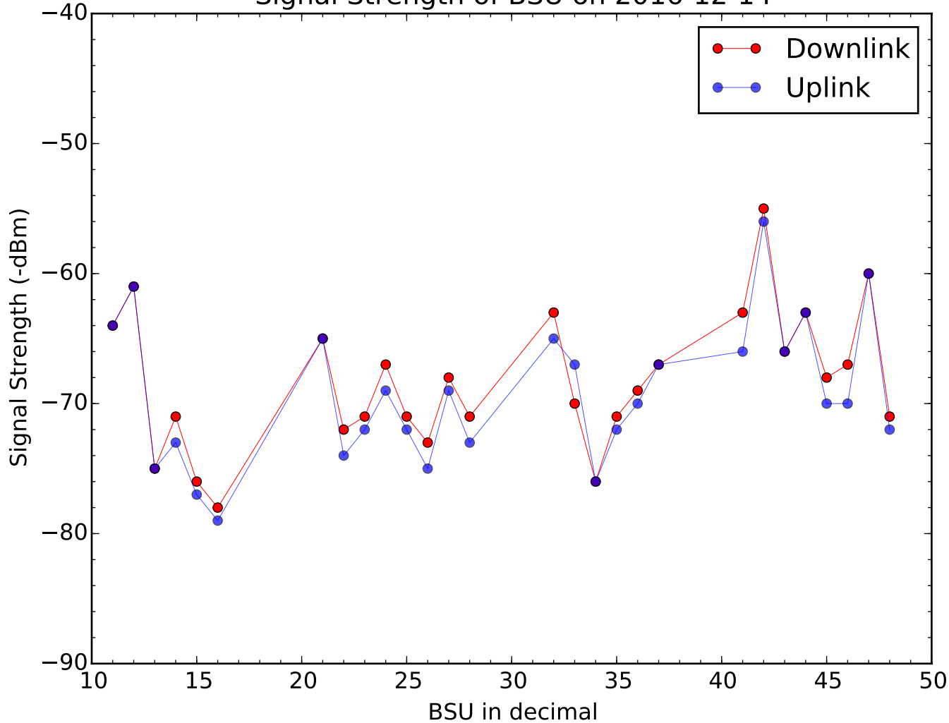
Signal Strength of BSU on 2016-12-14
