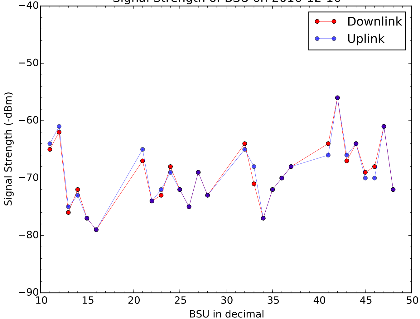
Signal Strength of BSU on 2016-12-16
