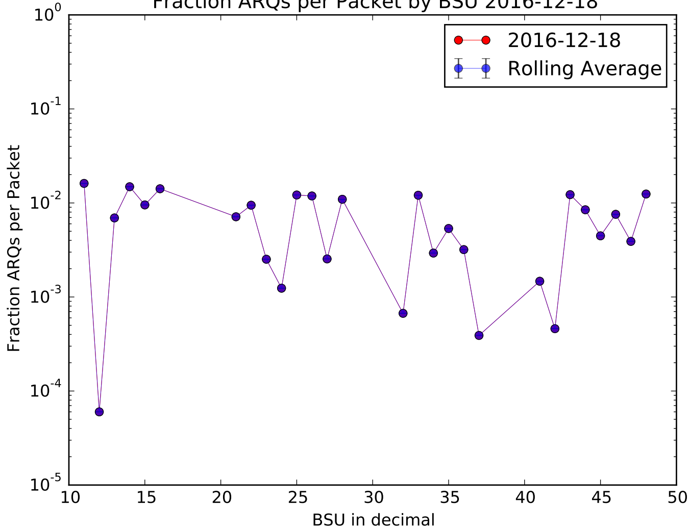
Fraction ARQs per Packet by BSU 2016-12-18
