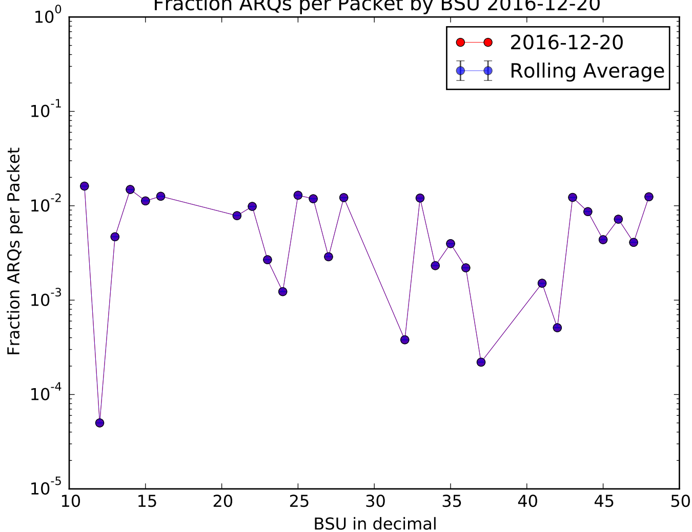
Fraction ARQs per Packet by BSU 2016-12-20
