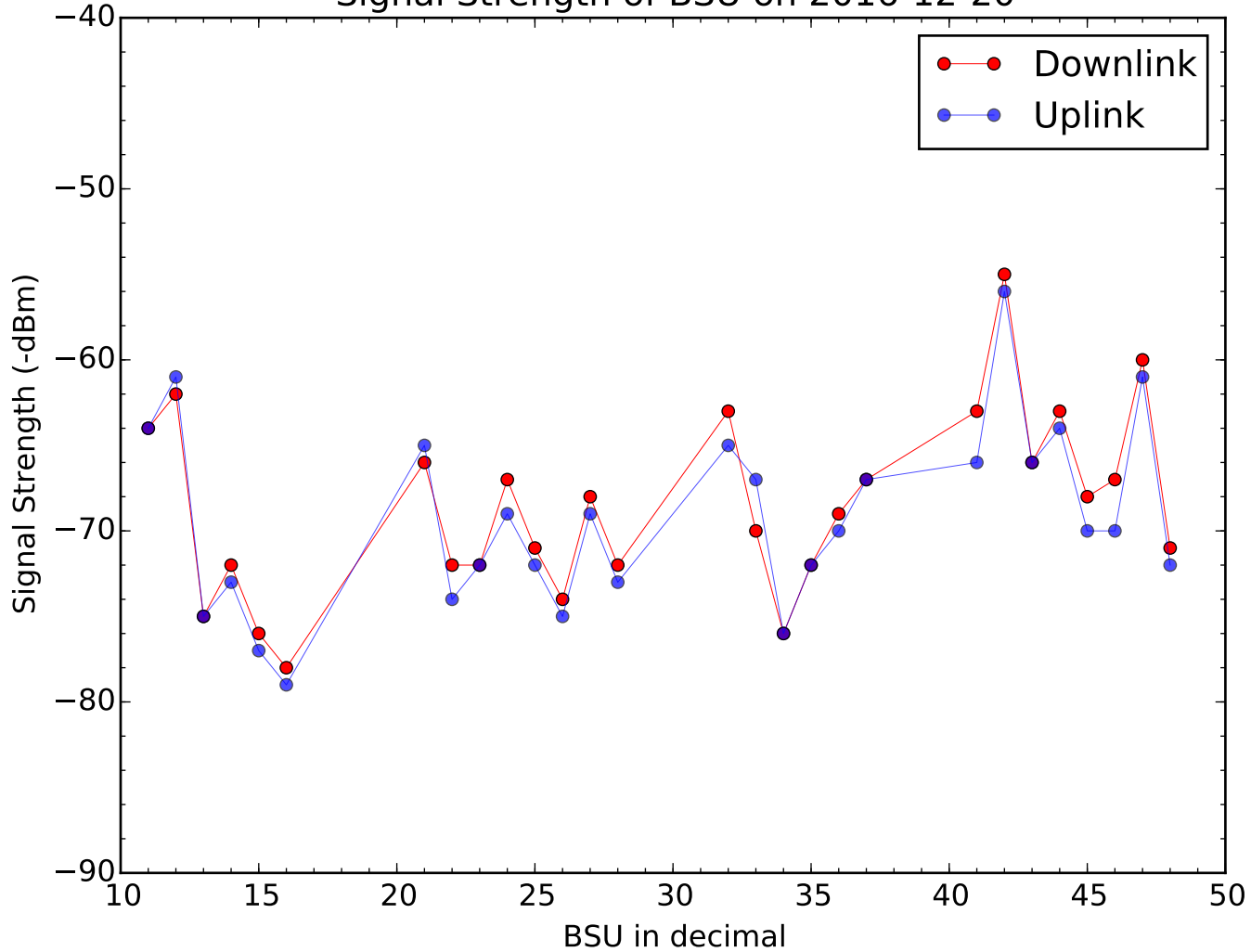
Signal Strength of BSU on 2016-12-20
