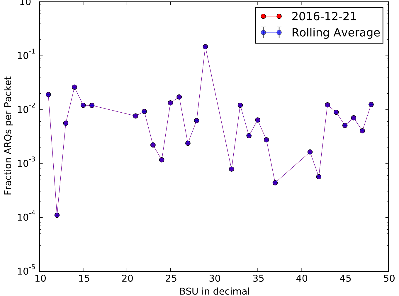
Fraction ARQs per Packet by BSU 2016-12-21
