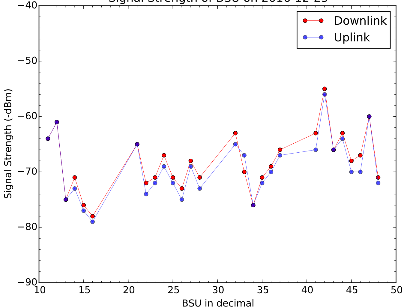
Signal Strength of BSU on 2016-12-23
