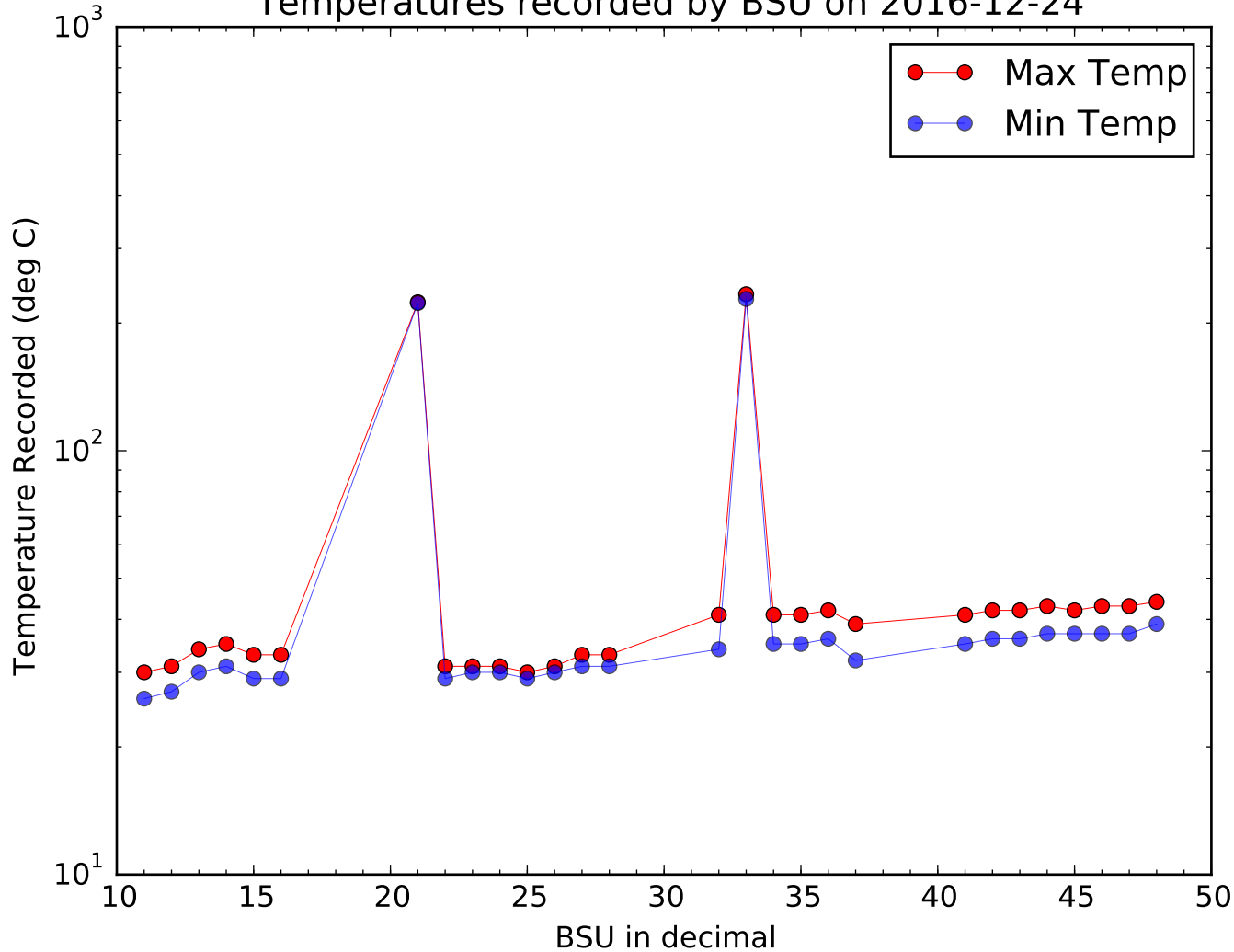
Temperatures recorded by BSU on 2016-12-24
