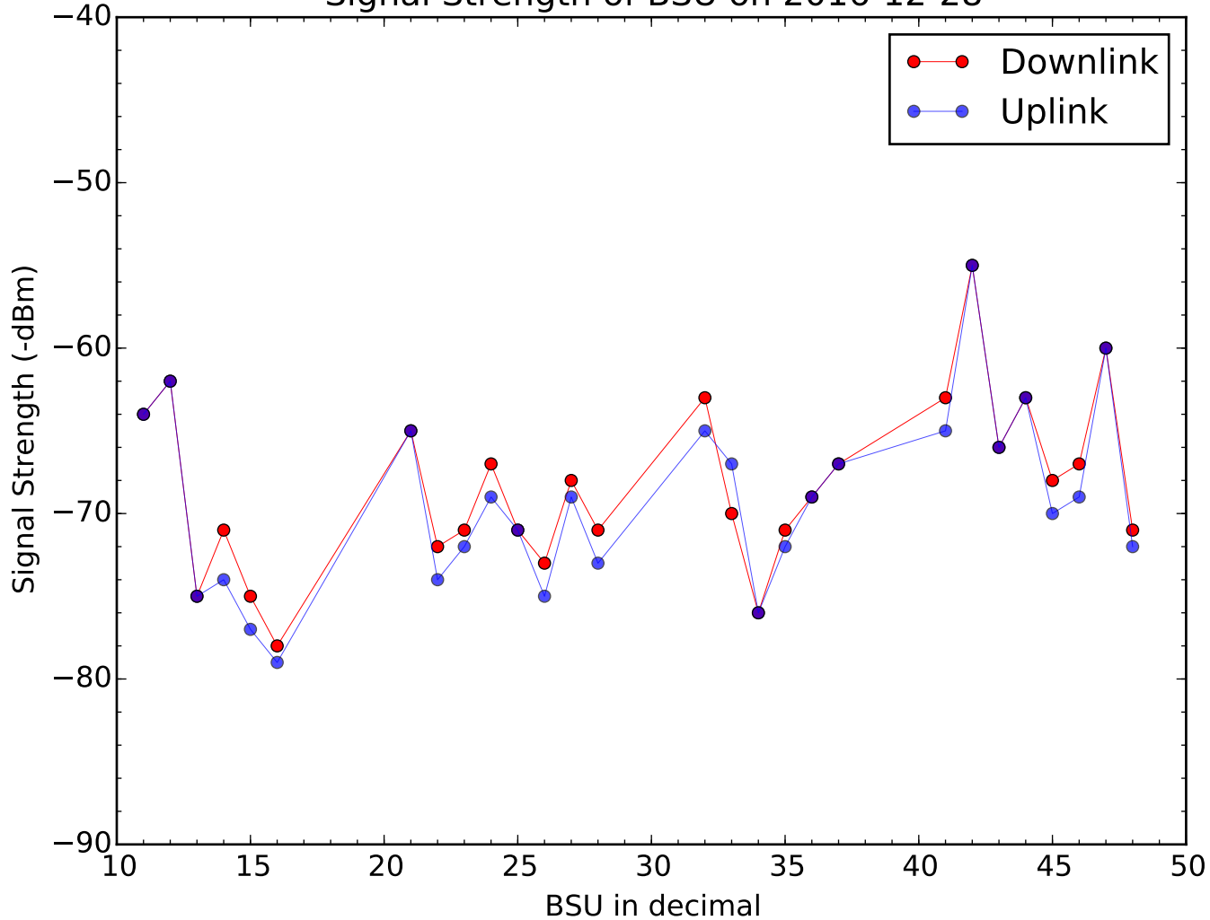
Signal Strength of BSU on 2016-12-28
