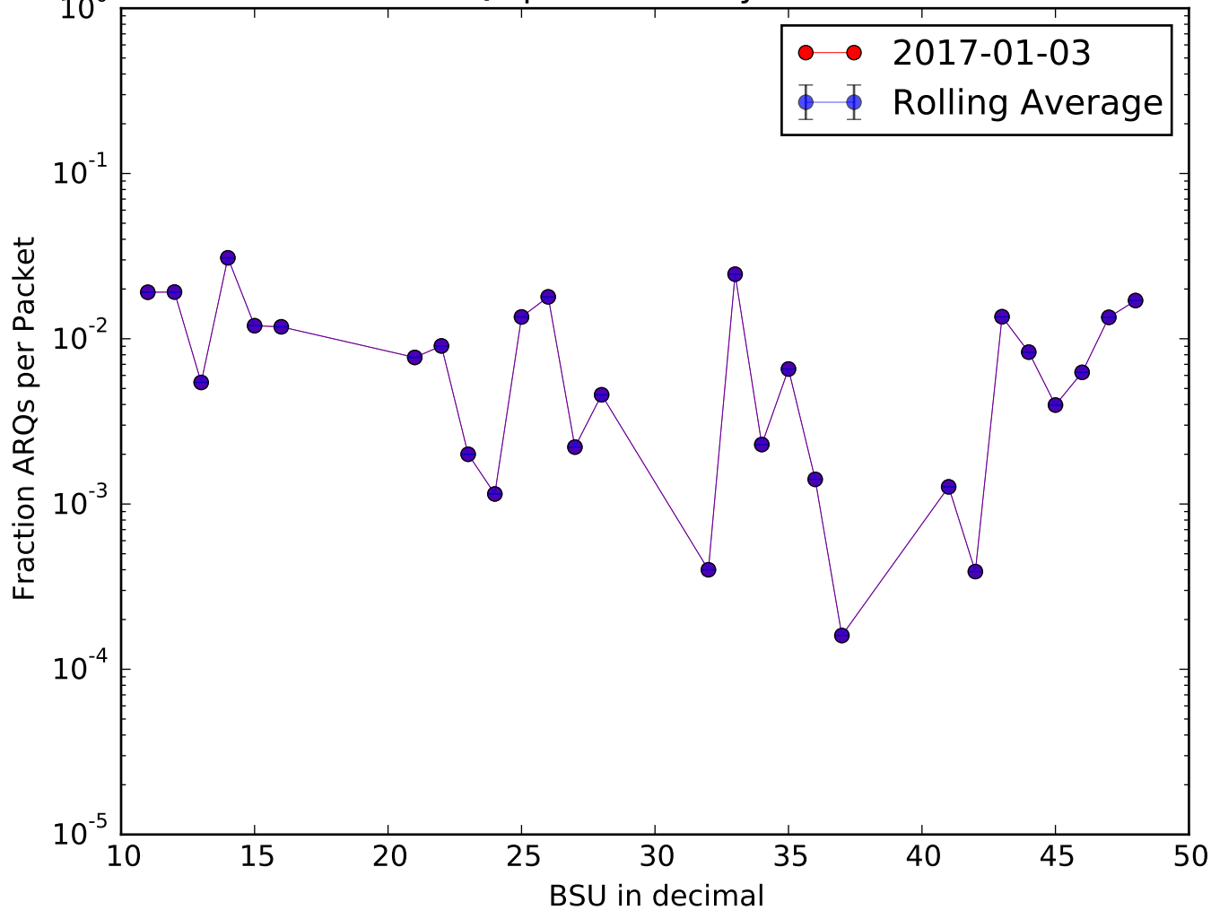
Fraction ARQs per Packet by BSU 2017-01-03
