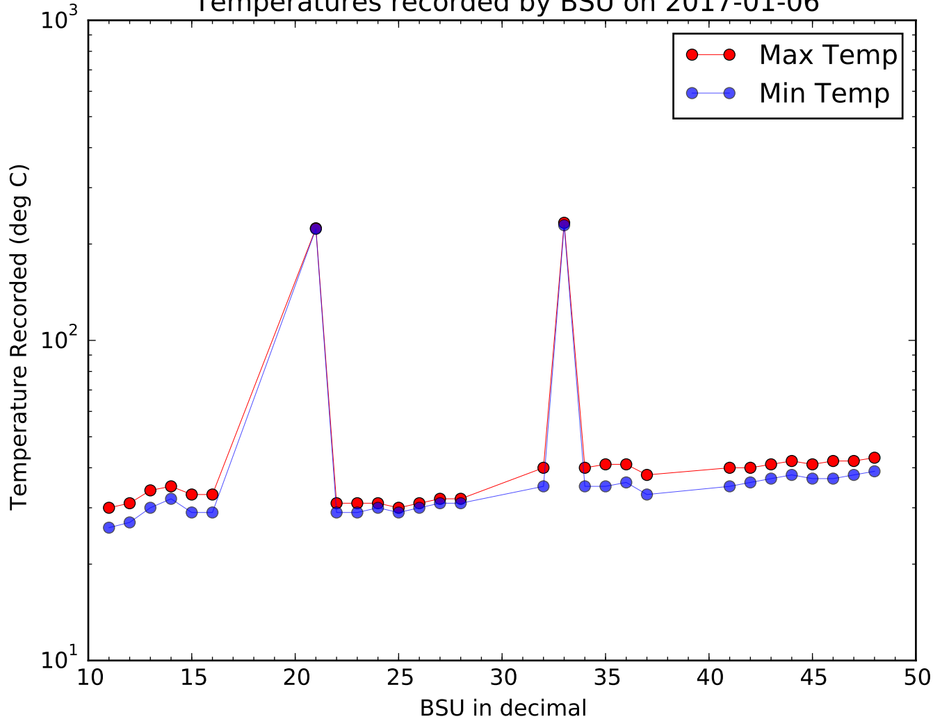
Temperatures recorded by BSU on 2017-01-06
