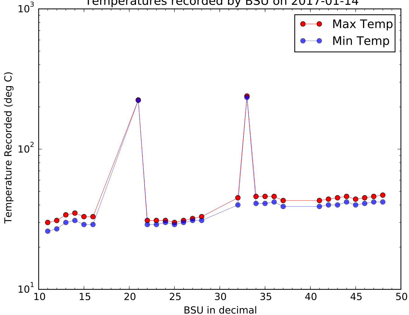
Temperatures recorded by BSU on 2017-01-14
