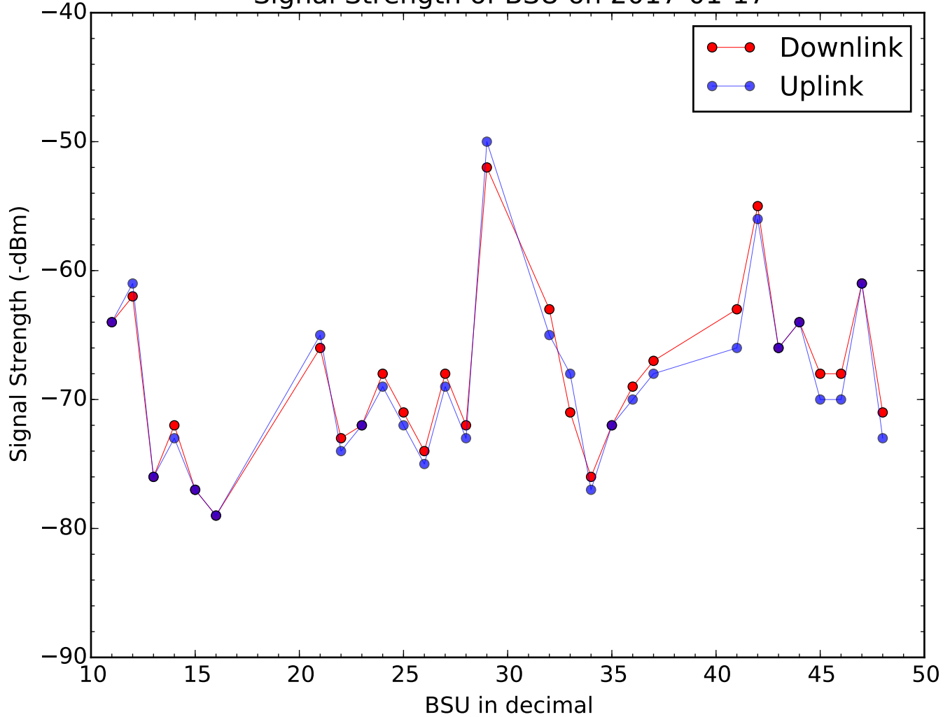
Signal Strength of BSU on 2017-01-17
