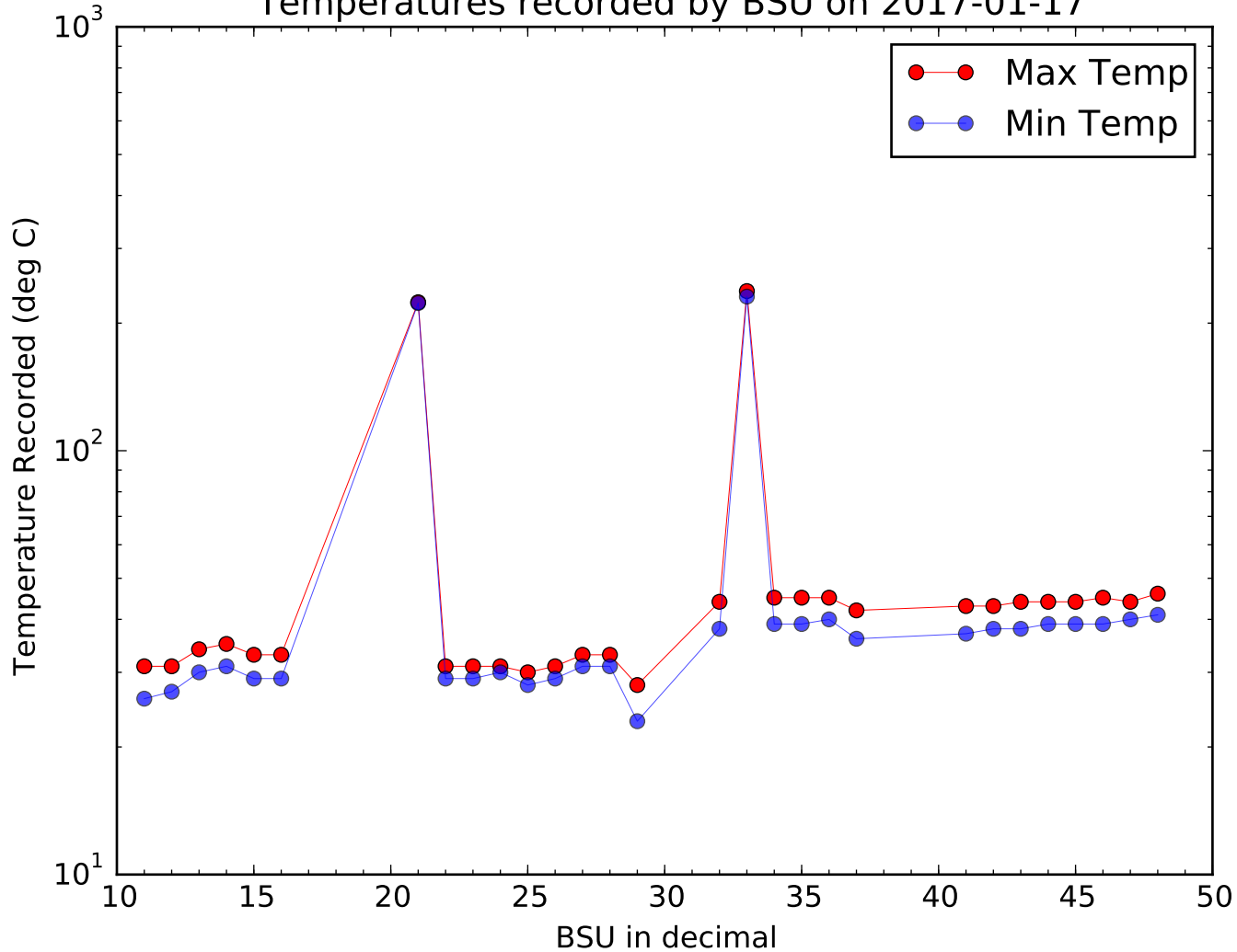
Temperatures recorded by BSU on 2017-01-17
