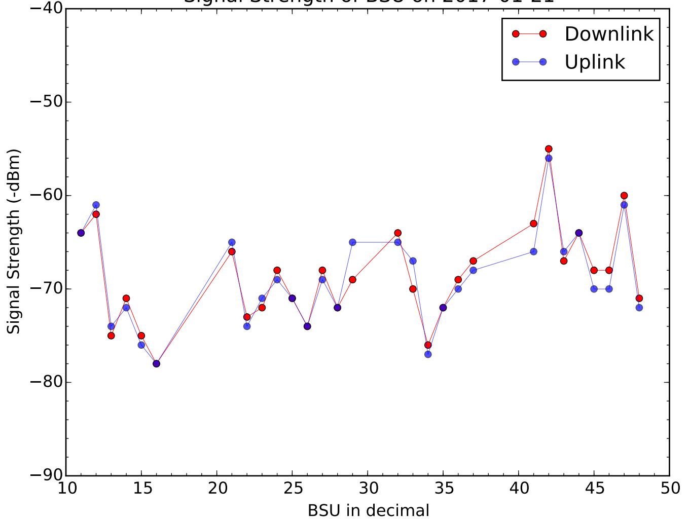
Signal Strength of BSU on 2017-01-21
