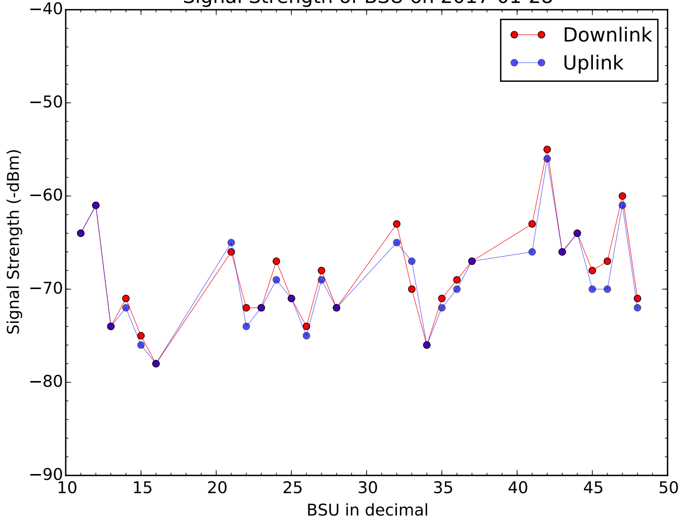
Signal Strength of BSU on 2017-01-28
