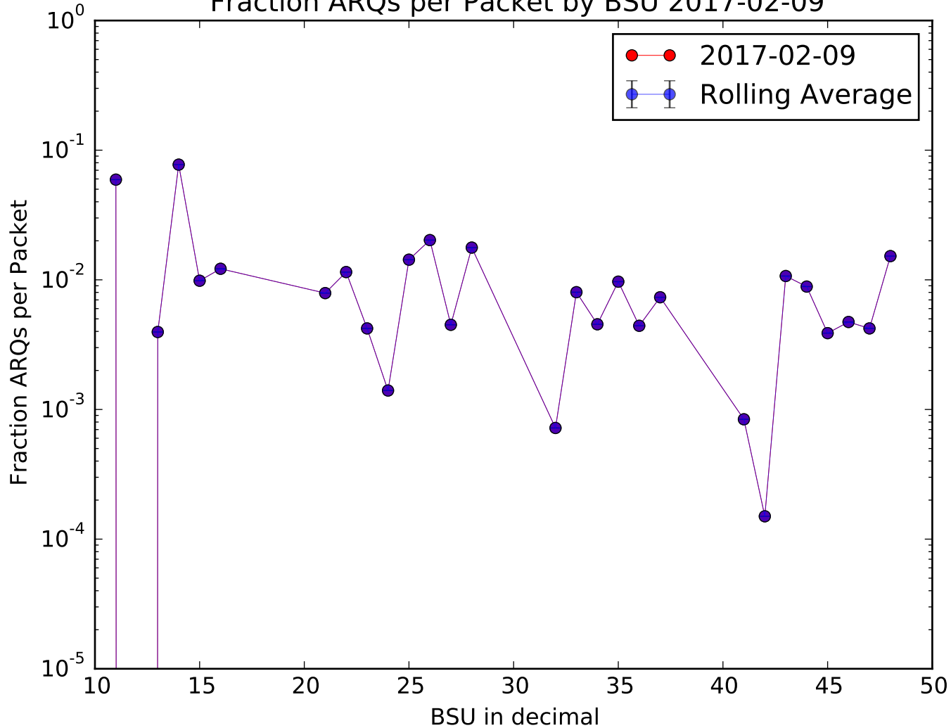
Fraction ARQs per Packet by BSU 2017-02-09
