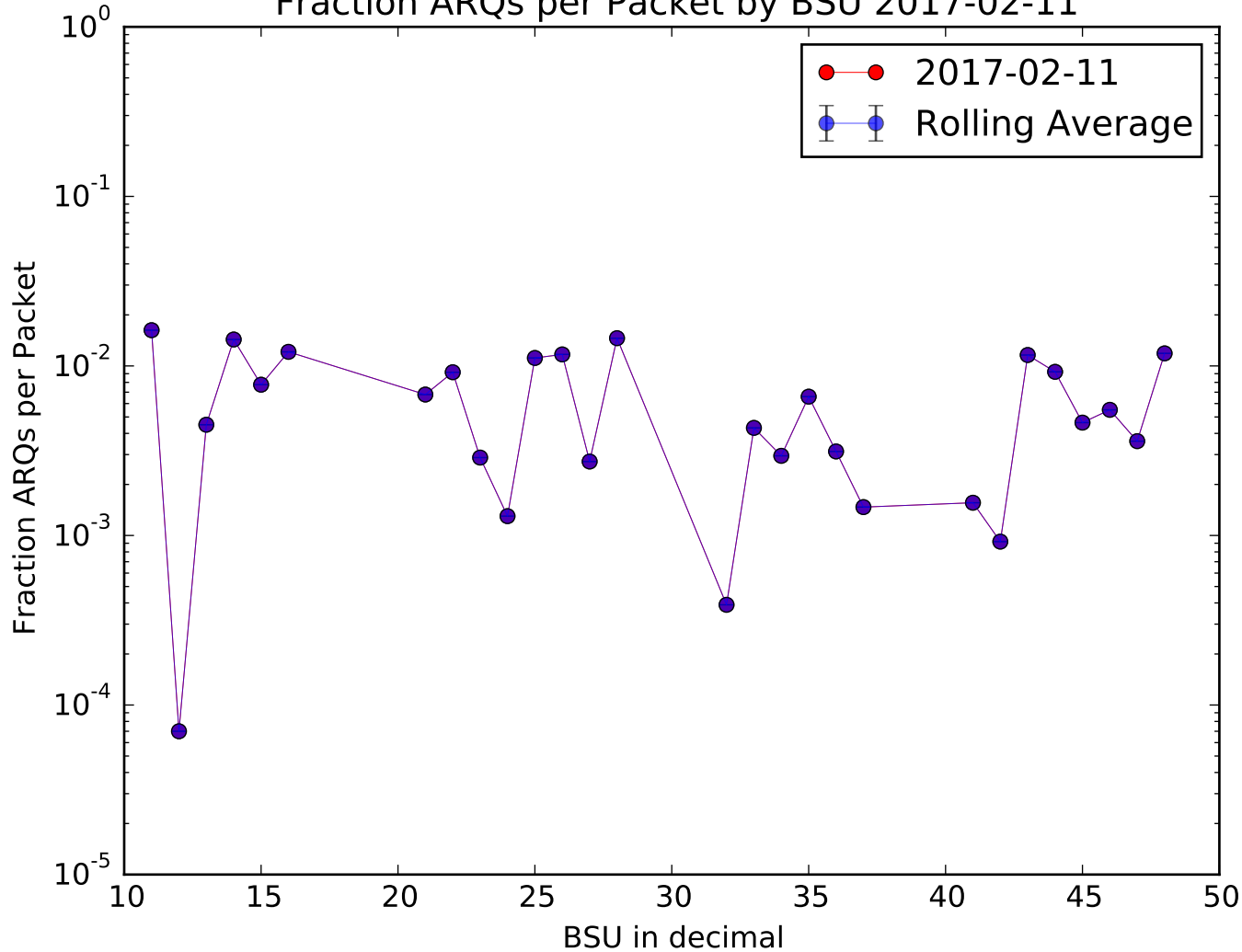
Fraction ARQs per Packet by BSU 2017-02-11
