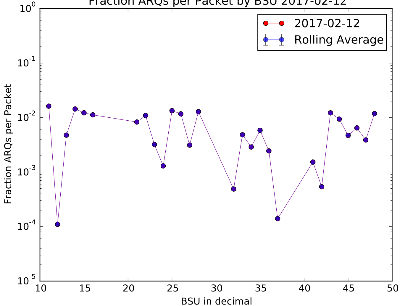
Fraction ARQs per Packet by BSU 2017-02-12
