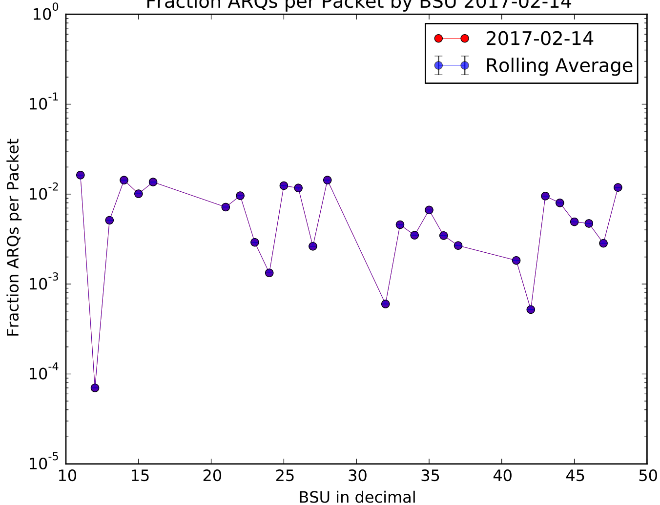
Fraction ARQs per Packet by BSU 2017-02-14
