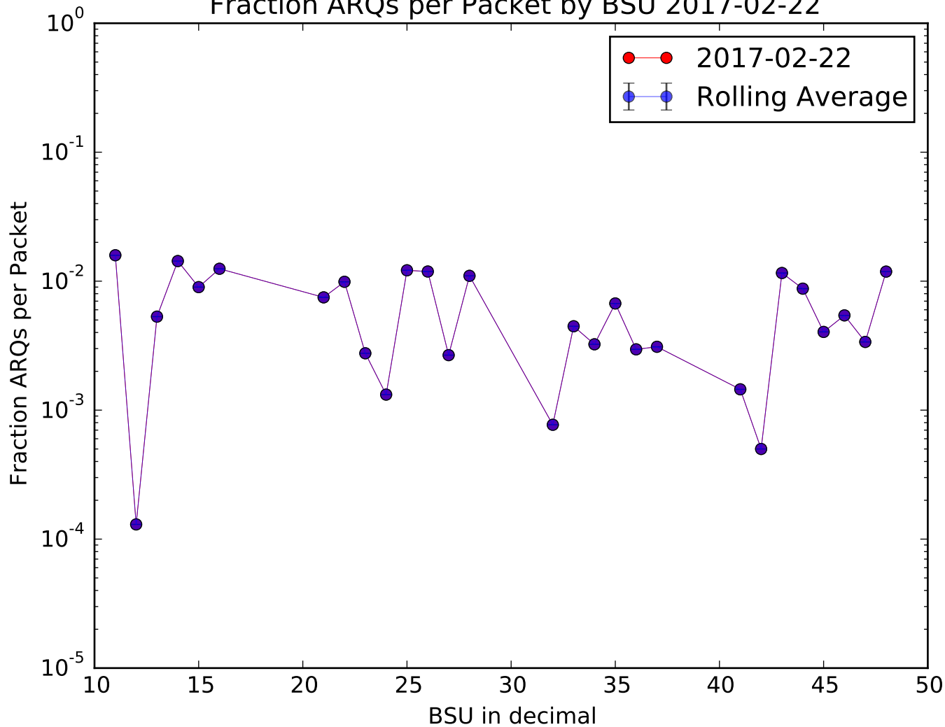
Fraction ARQs per Packet by BSU 2017-02-22
