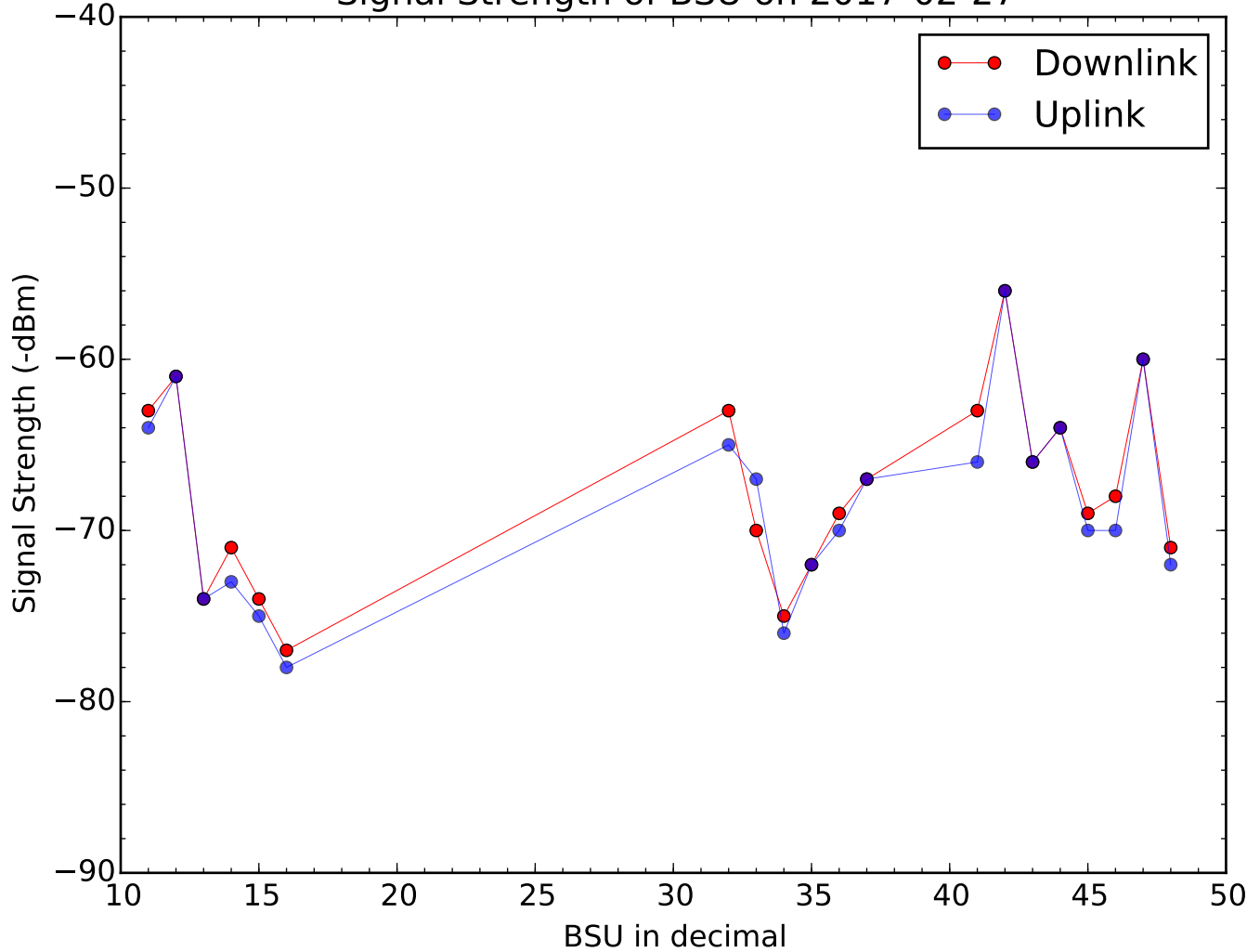
Signal Strength of BSU on 2017-02-27
