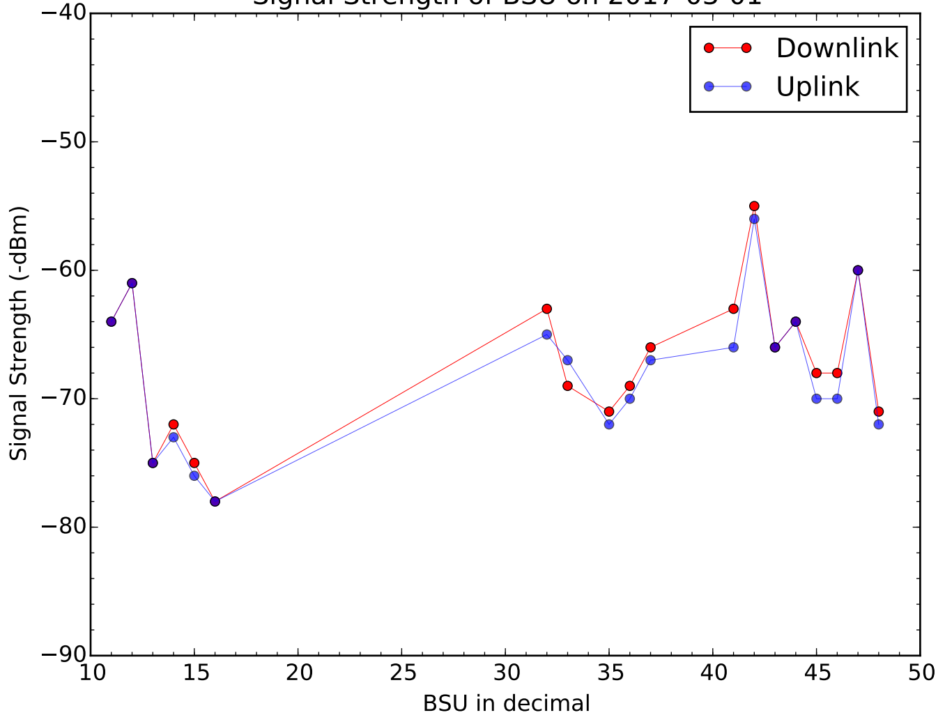
Signal Strength of BSU on 2017-03-01
