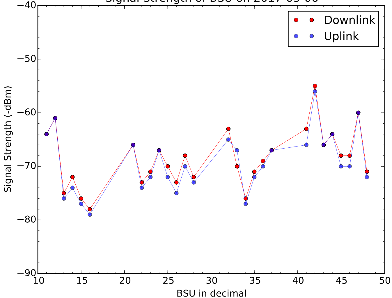
Signal Strength of BSU on 2017-03-06
