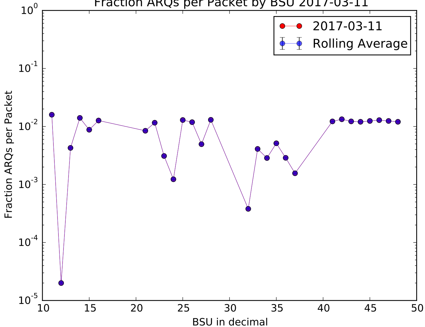
Fraction ARQs per Packet by BSU 2017-03-11
