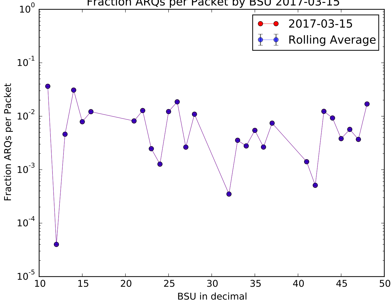
Fraction ARQs per Packet by BSU 2017-03-15
